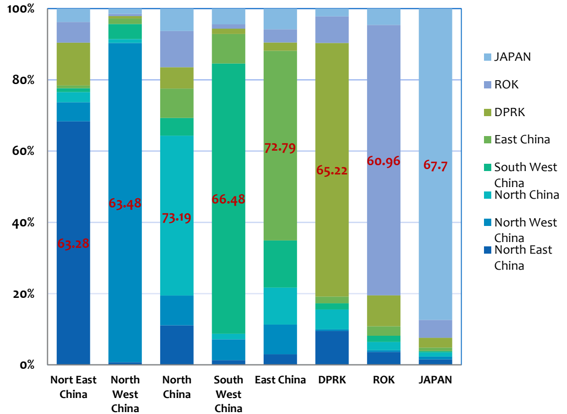
Annual average of PM 2.5 SRR
