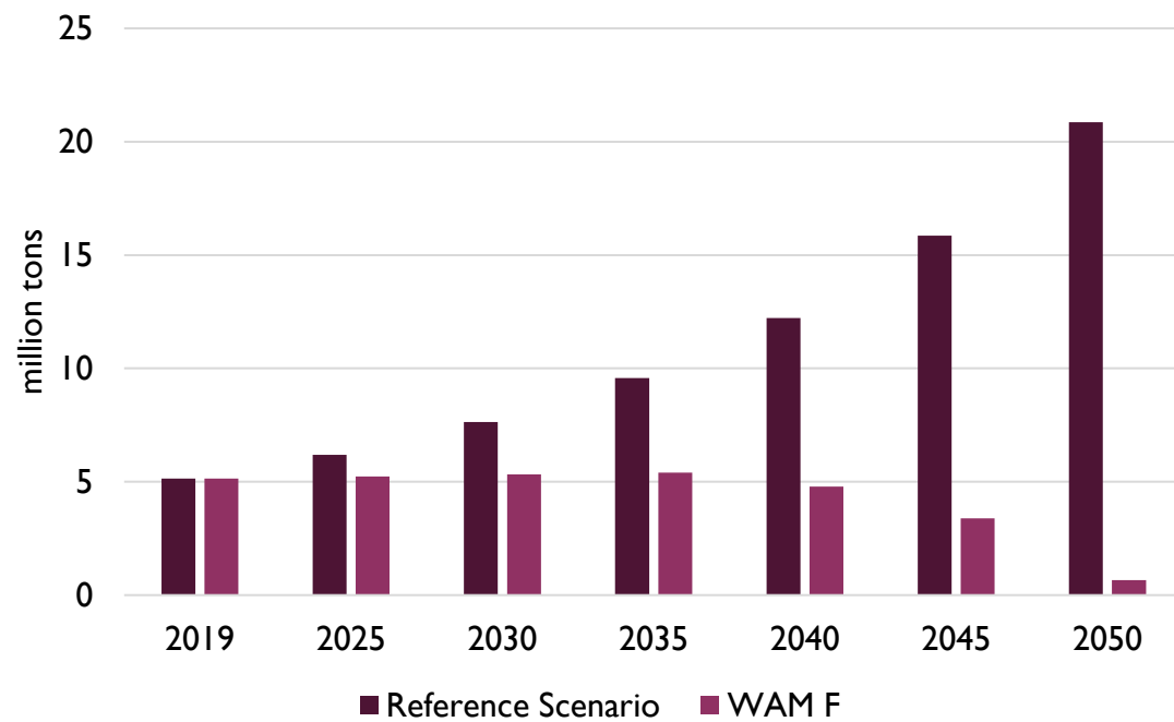
GHG emissions
